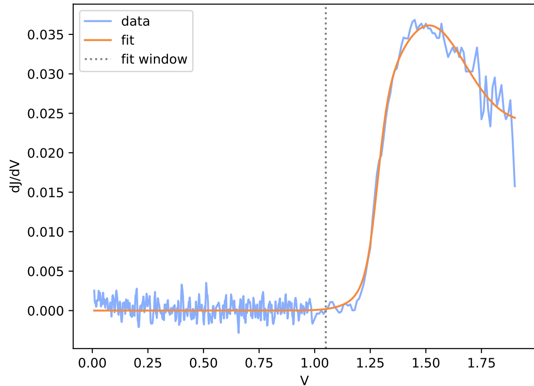
Run12-spot43.DTA.csv (window R^2 = 0.984 )
