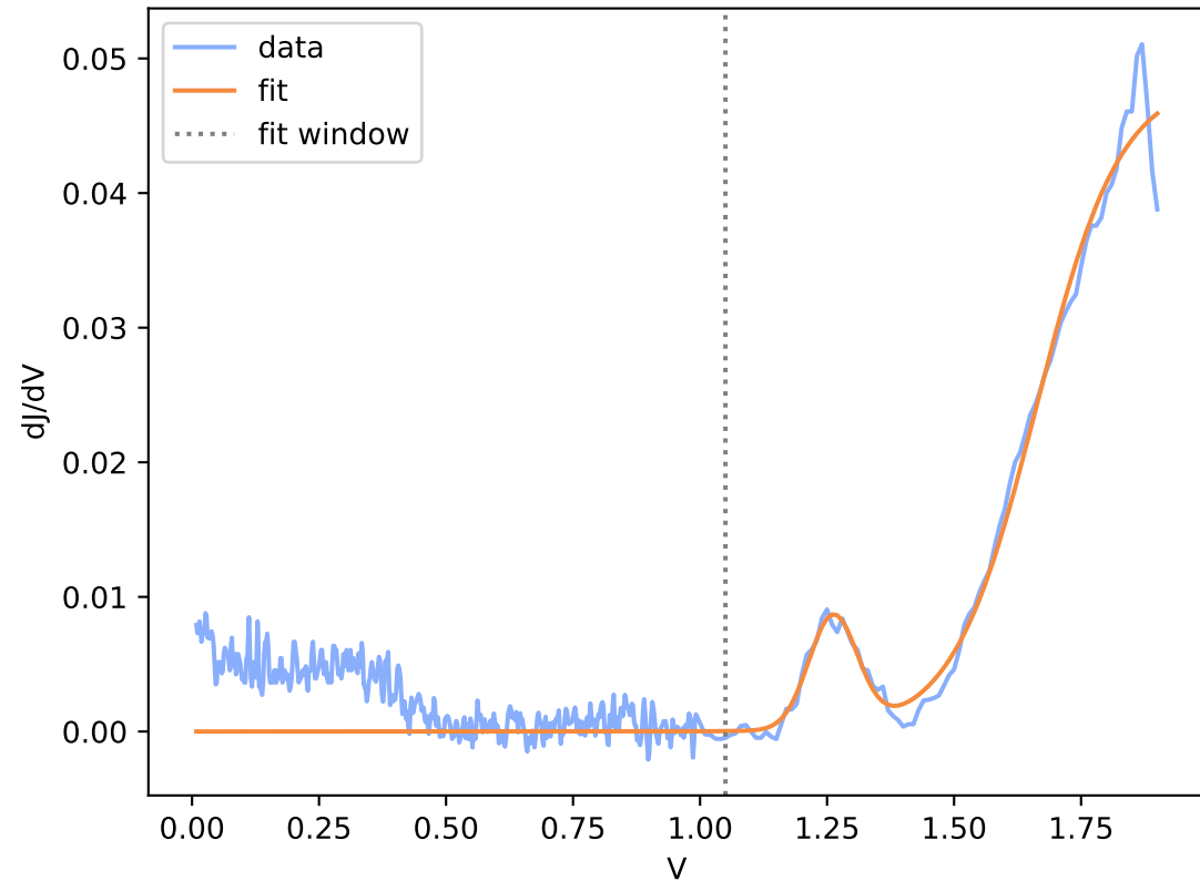
Run9-2-spot35.DTA.csv (window R^2 = 0.989 )
