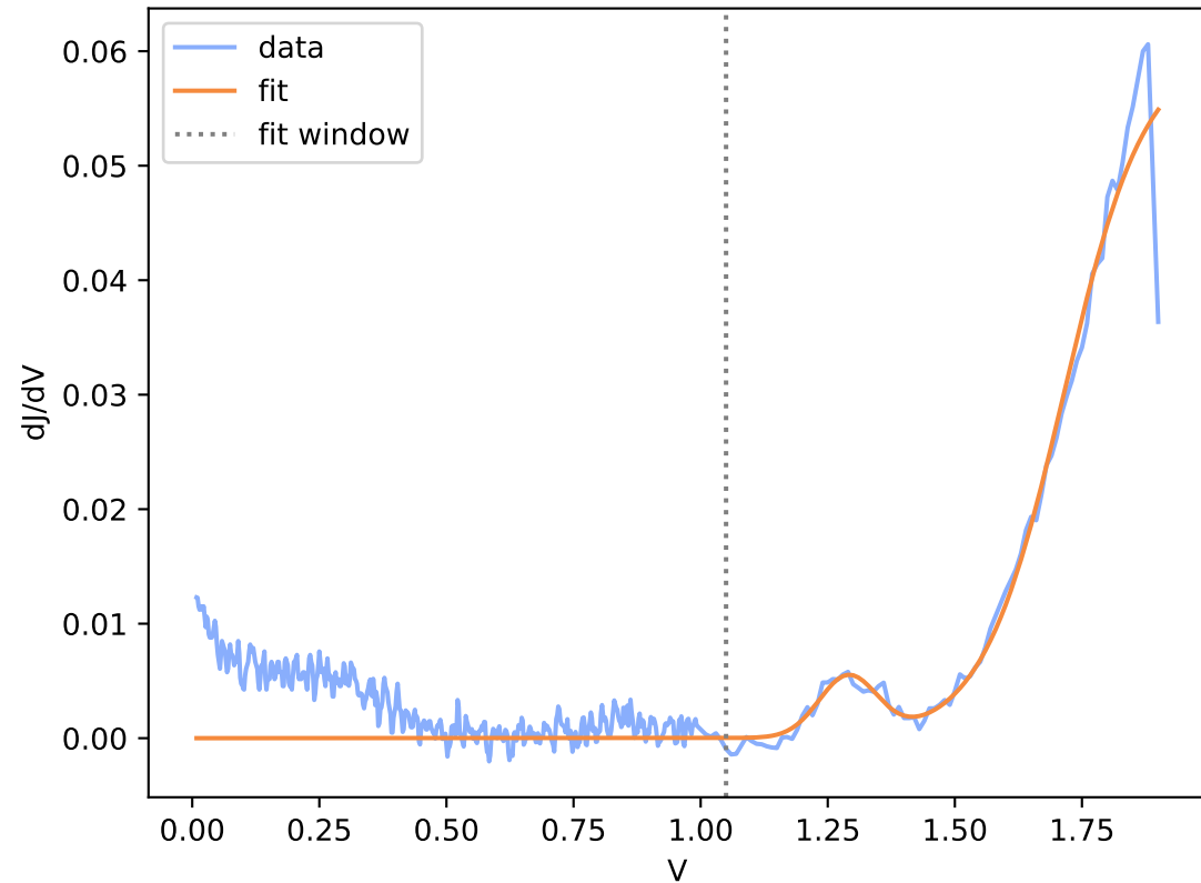
run11-2-spot13.DTA.csv (window R^2 = 0.978 )
