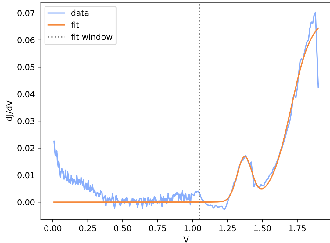
run11-2-spot16.DTA.csv (window R^2 = 0.976 )
