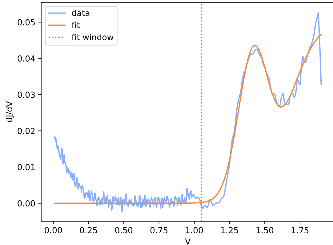
run11-2-spot5.DTA.csv (window R^2 = 0.975 )
