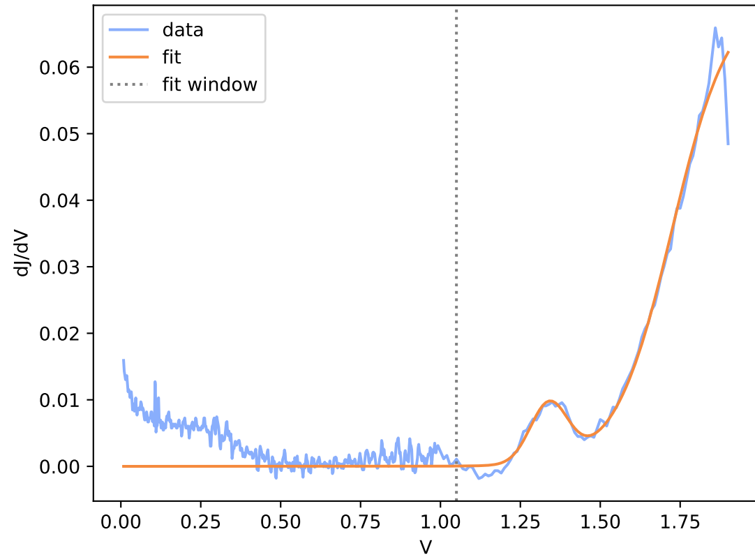
run9-2-spot16.DTA.csv (window R^2 = 0.989 )
