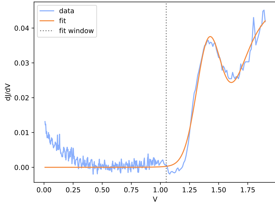
run9-2-spot19.DTA.csv (window R^2 = 0.979 )
