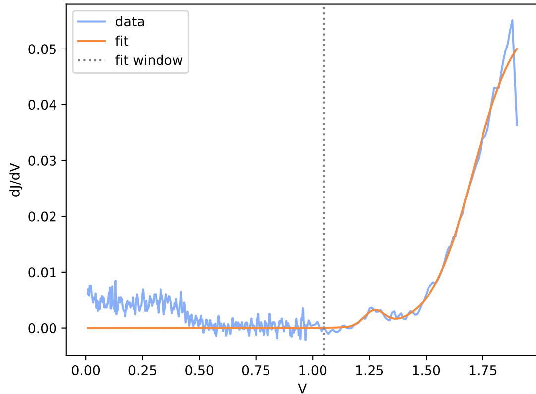
run9-2-spot28.DTA.csv (window R^2 = 0.986 )
