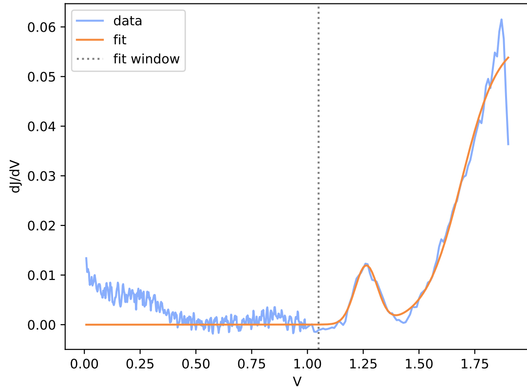
run9-2-spot6.DTA.csv (window R^2 = 0.975 )
