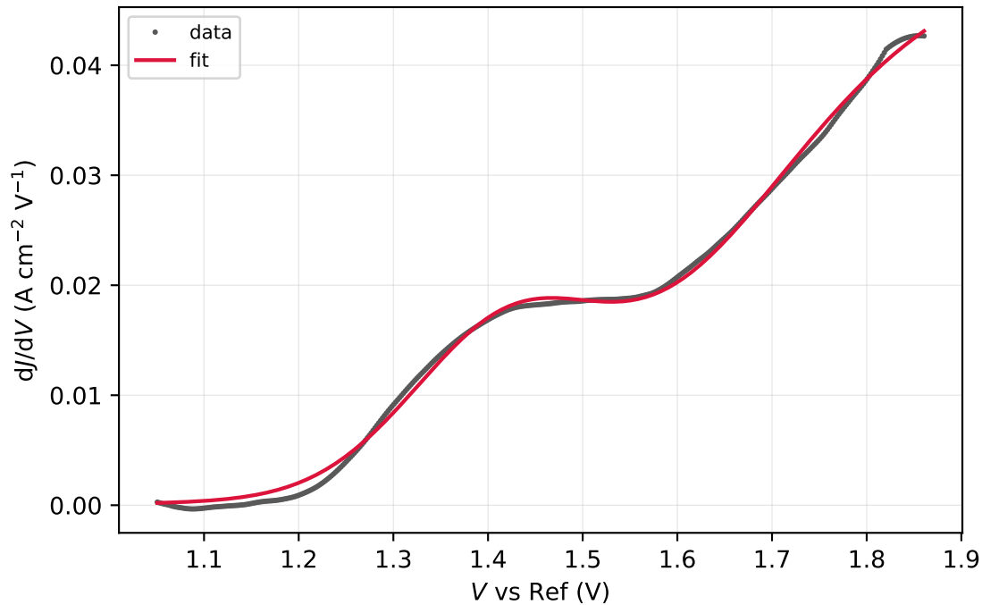
Run10-2-spot25.DTA.csv (window R^2 = 0.9981 )
