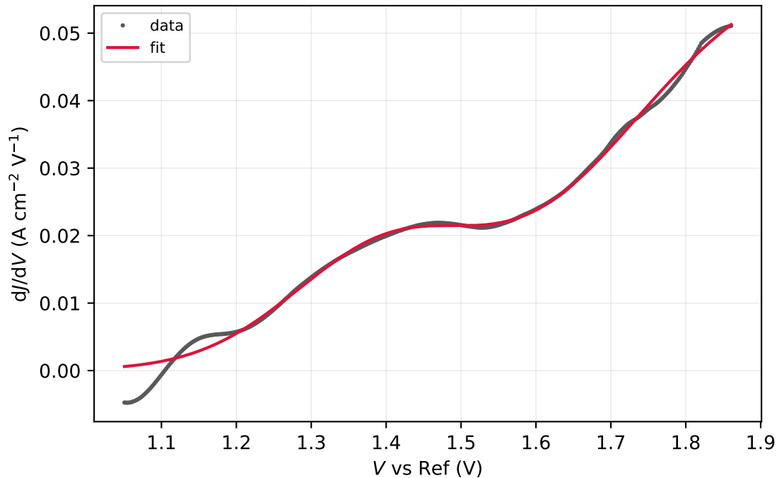
Run10-2-spot4.DTA.csv (window R^2 = 0.9921 )
