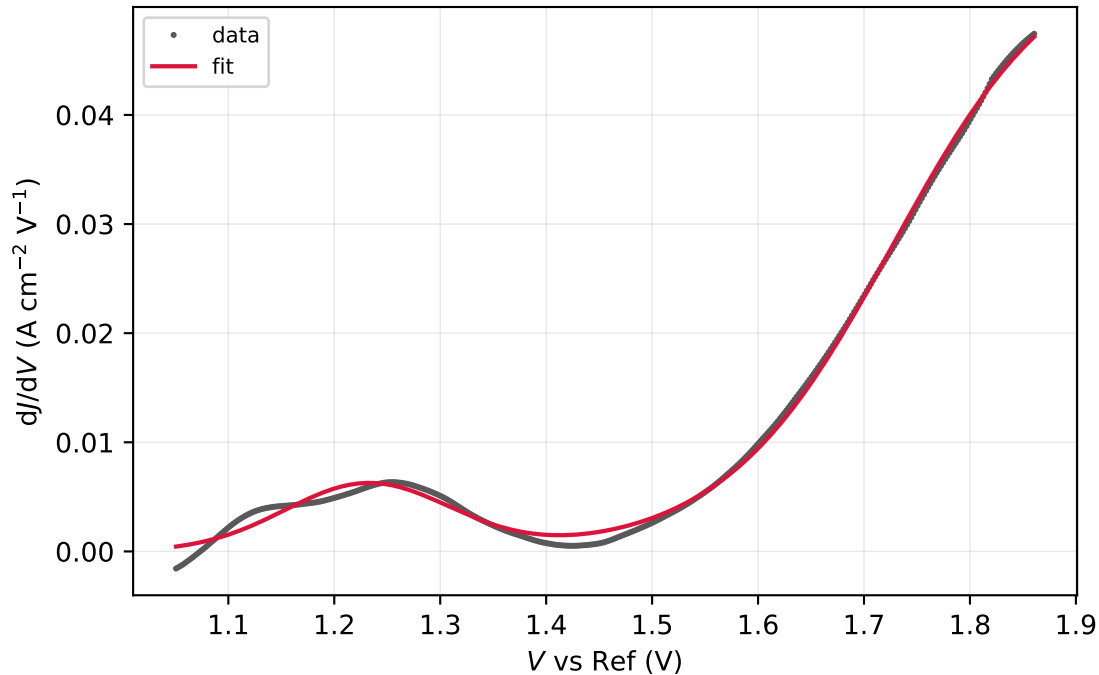
Run10-2-spot6.DTA.csv (window R^2 = 0.9980 )
