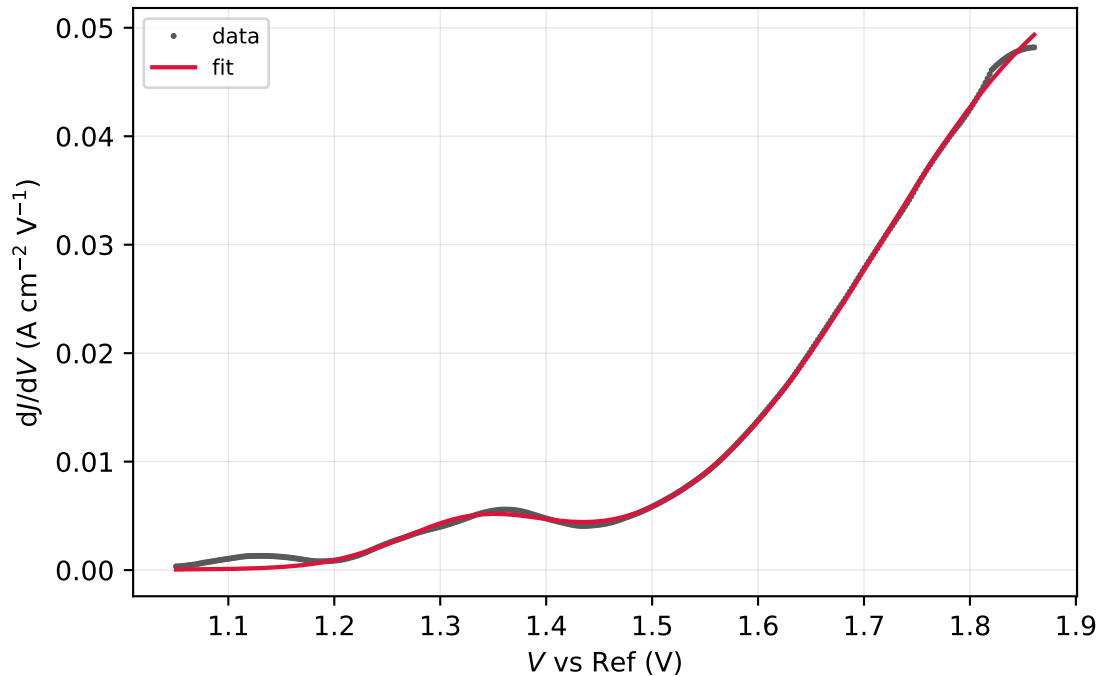
Run10-2-spot8.DTA.csv (window R^2 = 0.9993 )
