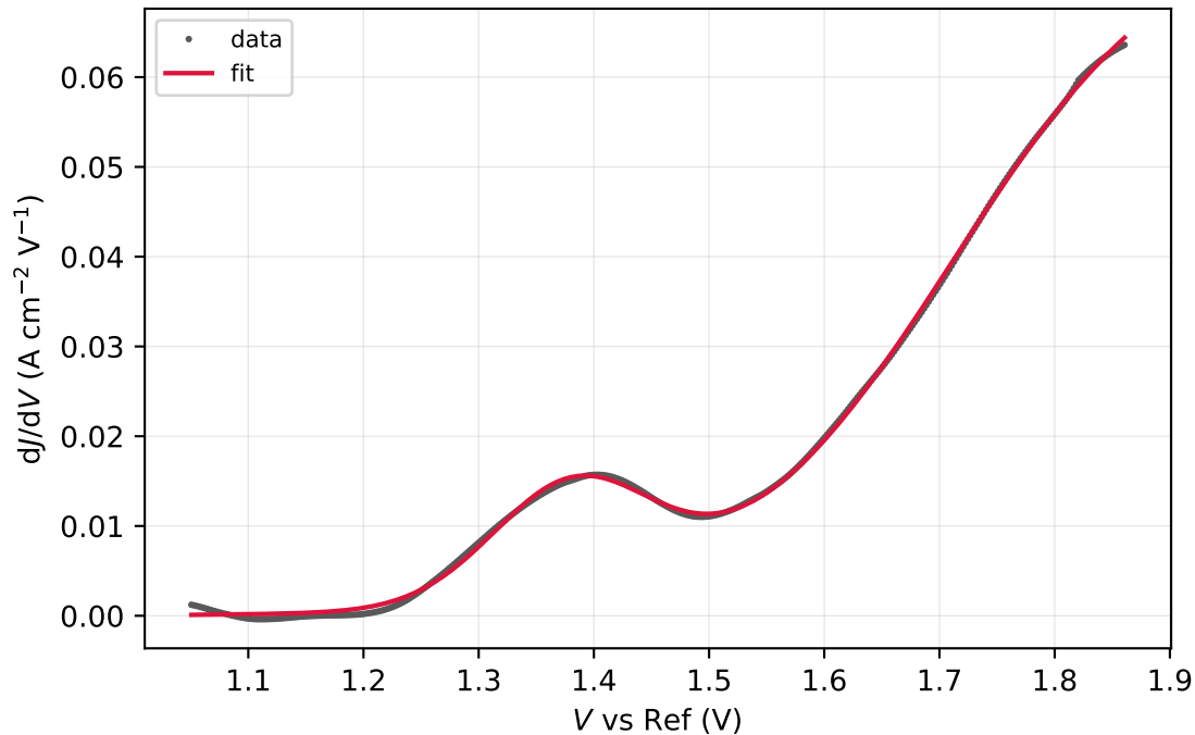
Run9-2-spot40.DTA.csv (window R^2 = 0.9996 )
