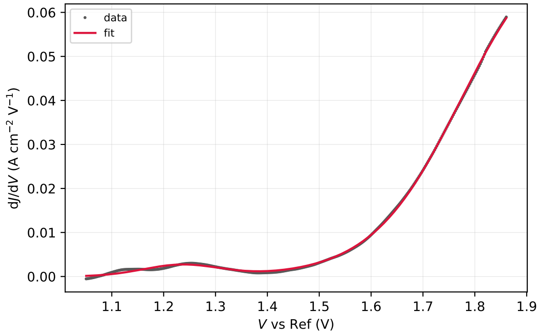
run9-2-spot21.DTA.csv (window R^2 = 0.9997 )
