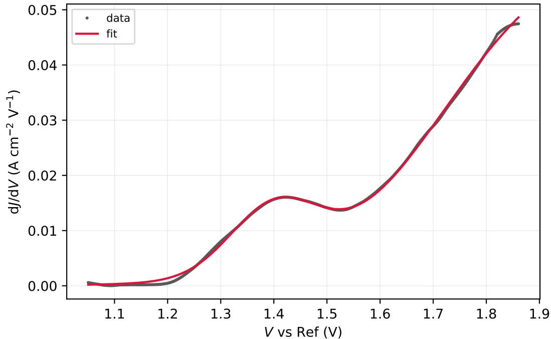
Run10-2-spot32.DTA.csv (window R^2 = 0.9993 )
