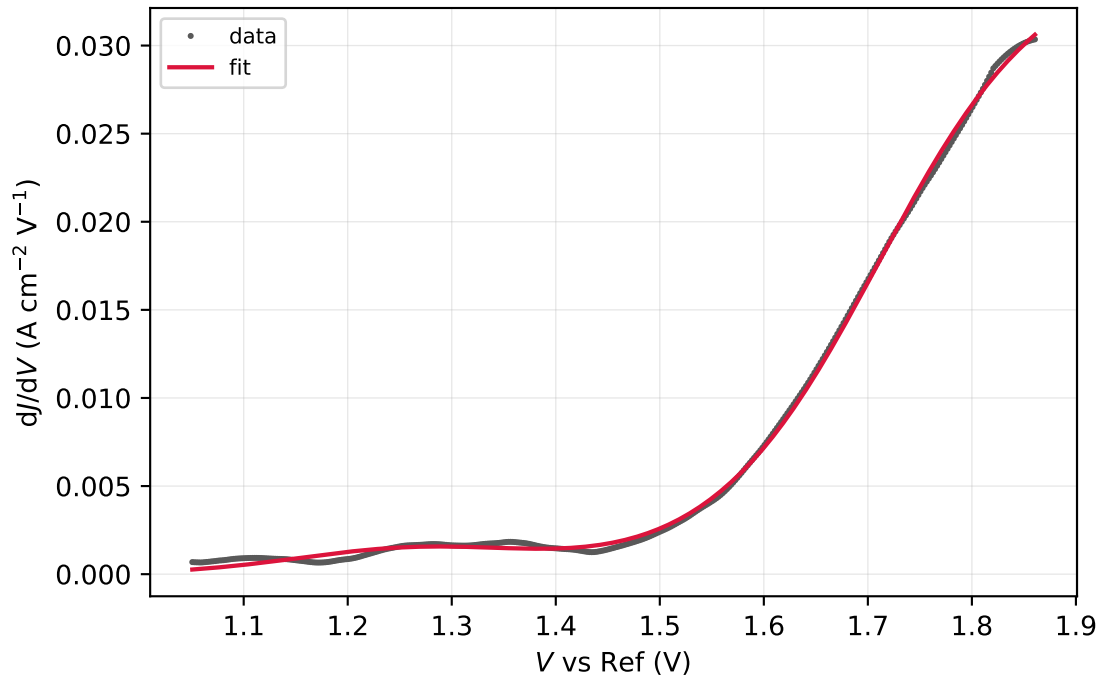
Run10-2-spot42.DTA.csv (window R^2 = 0.9993 )
