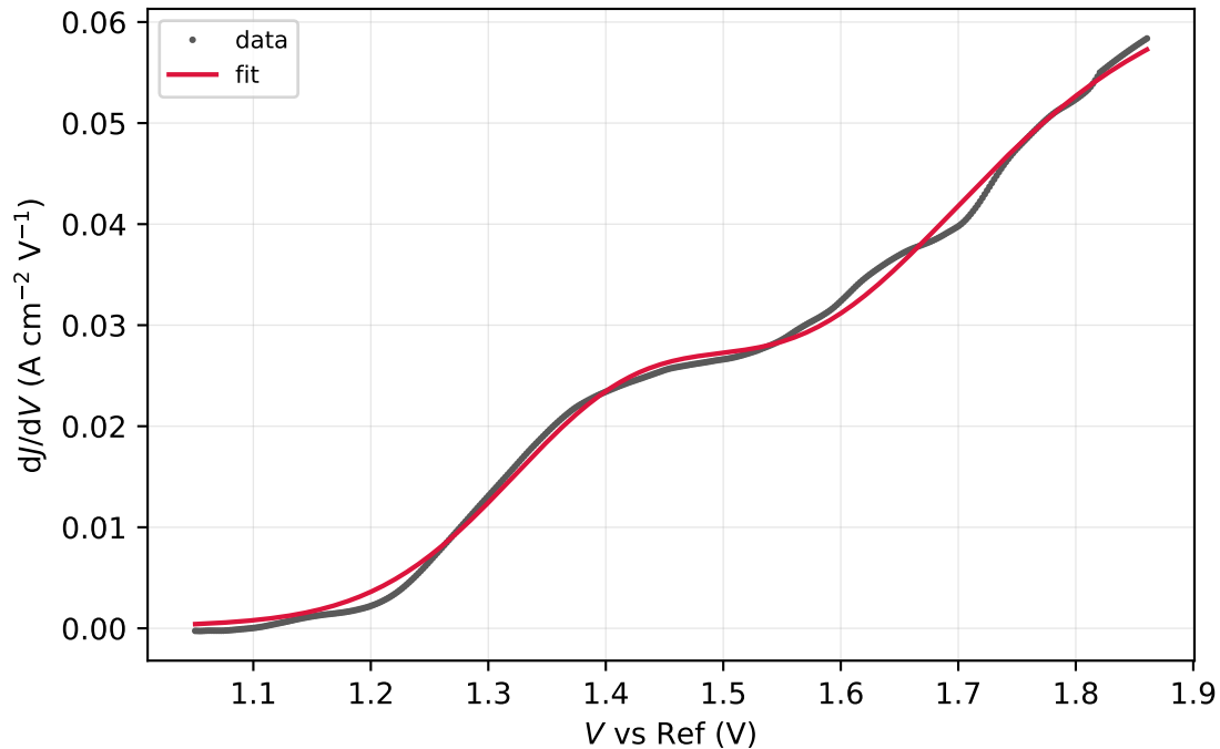
Run12-spot15.DTA.csv (window R^2 = 0.9975 )
