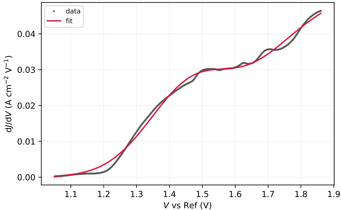
Run12-spot43.DTA.csv (window R^2 = 0.9954 )
