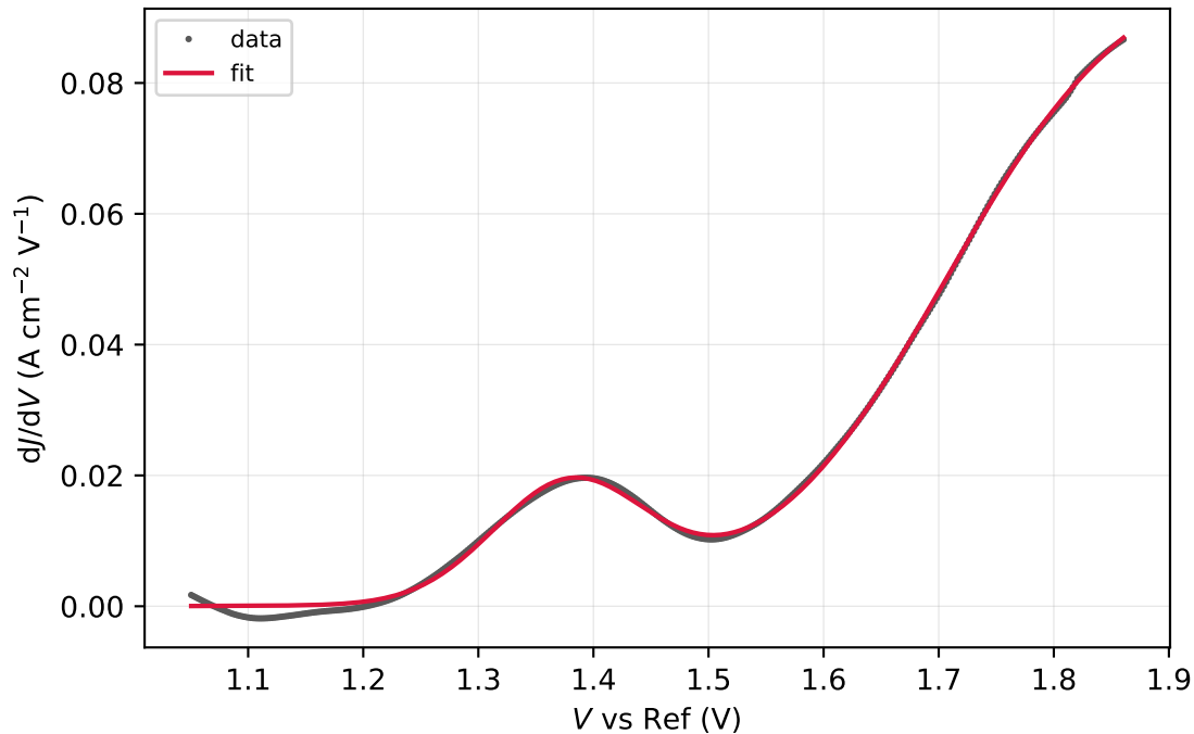
run11-2-spot24.DTA.csv (window R^2 = 0.9993 )
