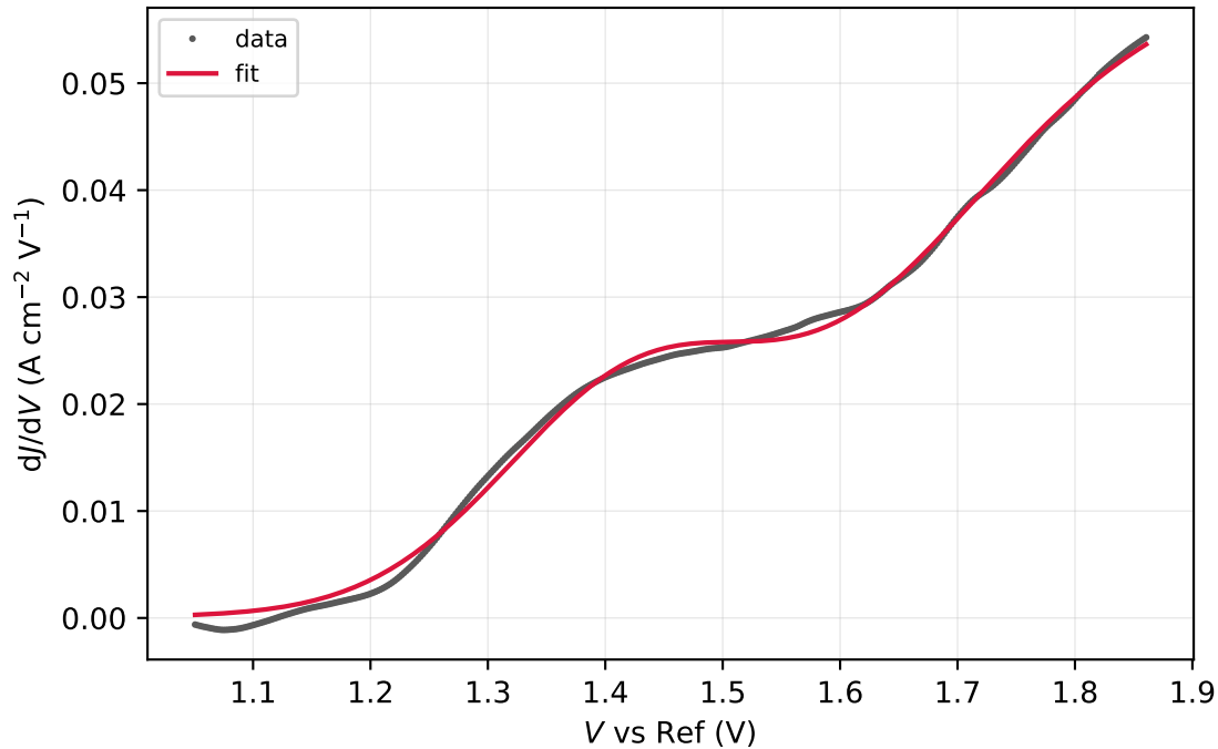
run9-2-spot19.DTA.csv (window R^2 = 0.9977 )
