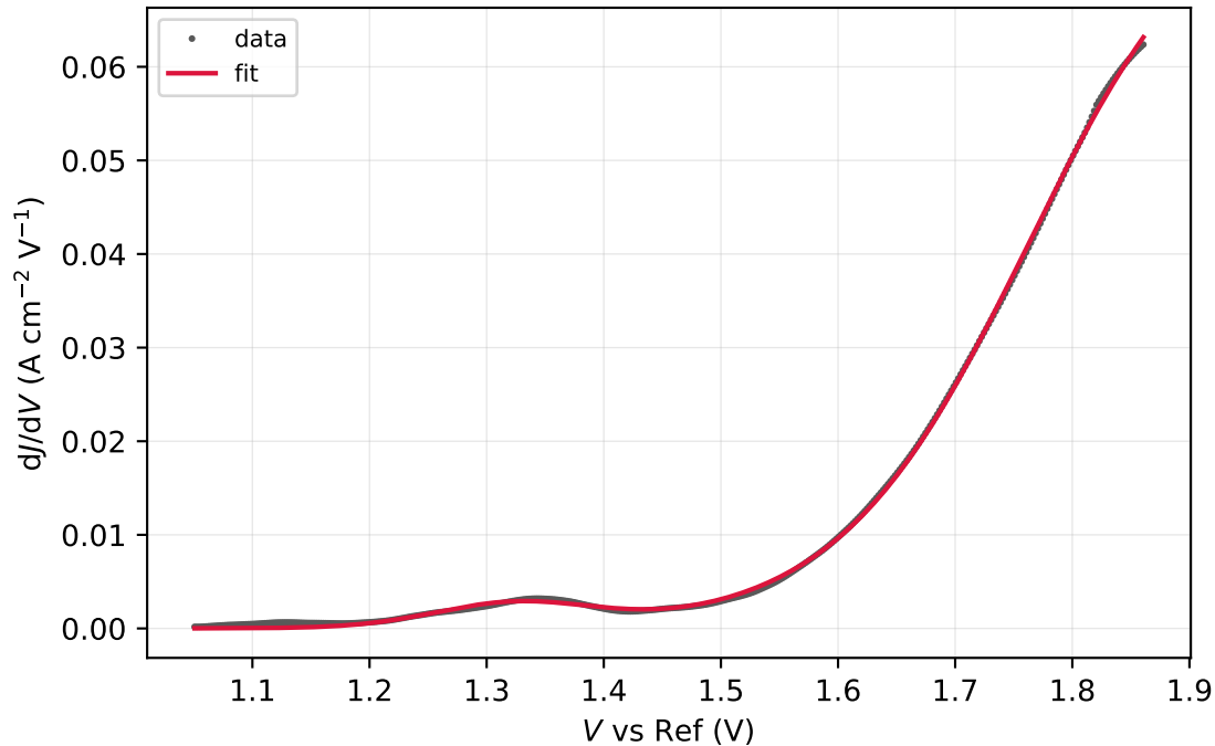
run9-2-spot23.DTA.csv (window R^2 = 0.9998 )
