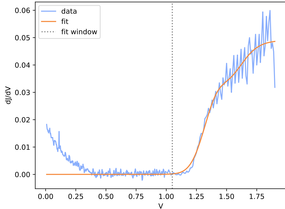
Run10-2-spot19.DTA.csv (window R^2 = 0.945 )
