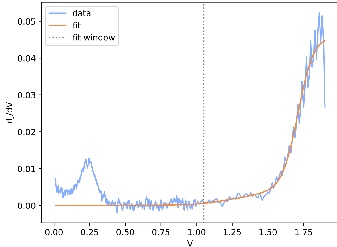
Run10-2-spot29.DTA.csv (window R^2 = 0.964 )
