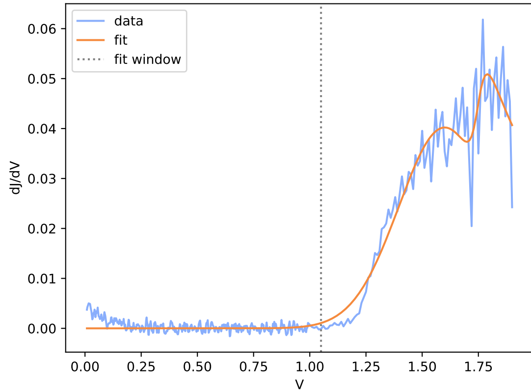
Run12-spot40.DTA.csv (window R^2 = 0.917 )
