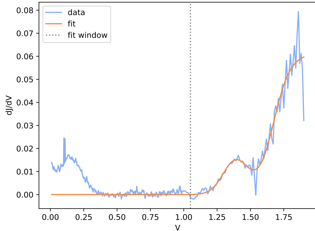
Run9-2-spot32.DTA.csv (window R^2 = 0.939 )
