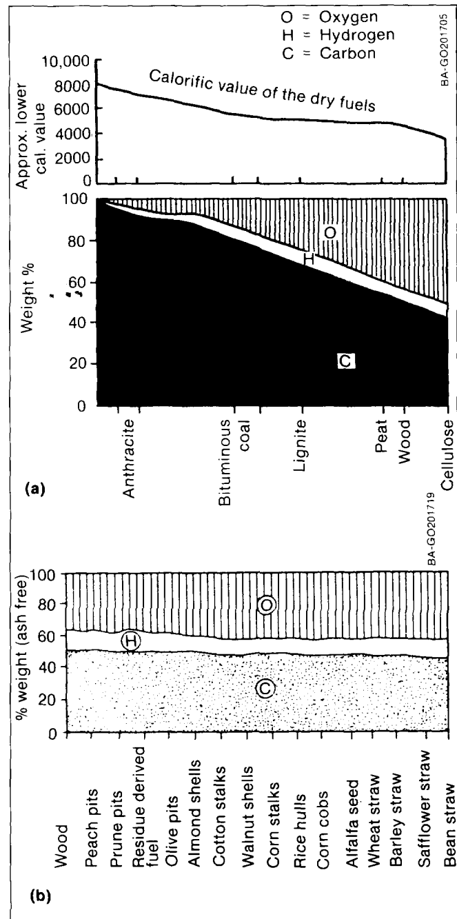
Fig. 3-1. Elemental (ultimate) analysis of (a) coals and wood and (b) biomass fuels (Sources: Skov 1974, p. 35. (©1974. Used with permission of Biomass Energy Foundation, Inc.) and Kaupp 1984a, Fig. 96)
