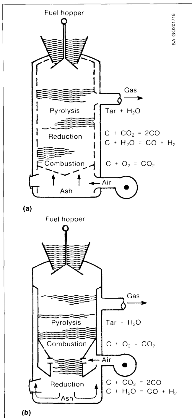
Fig. 4-5. Schematic diagram of (a) updraft and (b) downdraft gasifier showing reactions occurring in each zone (Source: Reed 1981, Figs. 8-6, 8-7)
