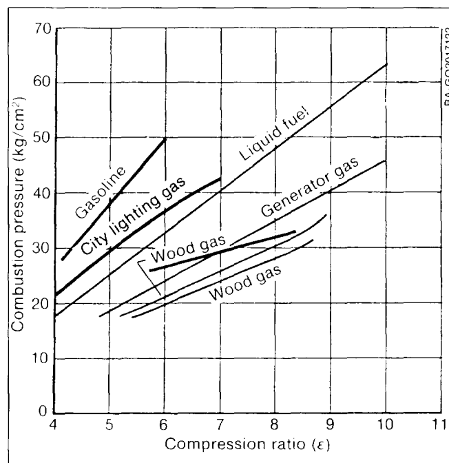
Fig. 11-16. Combustion pressure versus compression ratio for various fuels (Source: Gengas 1950, Fig. 174)
