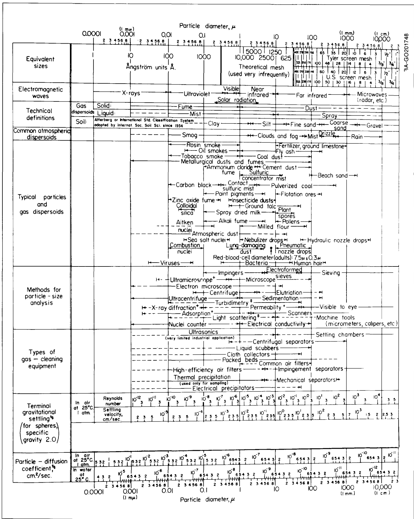
Fig. 7-6. Characteristics of particles and particle dispersoids (Source: Adapted from Perry 1973, Fig. 20-92)
