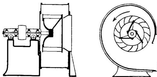
Backward-curved-blade fan.
