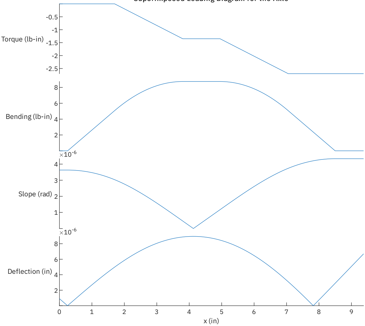
Superimposed Loading Diagram for the Axle
