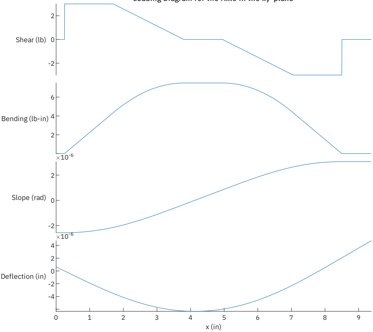
Loading Diagram for the Axle in the xy-plane
