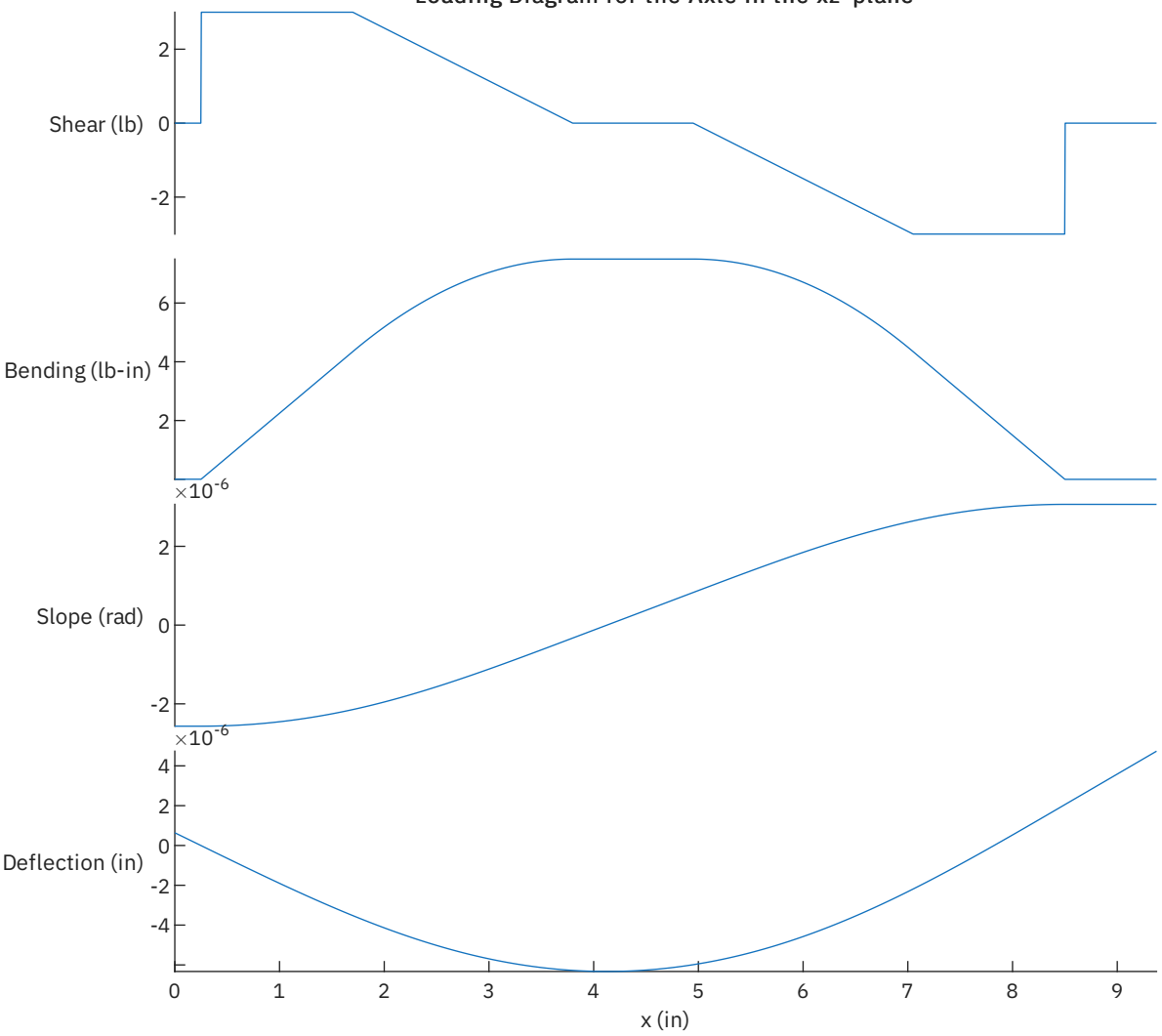
Loading Diagram for the Axle in the xz-plane
