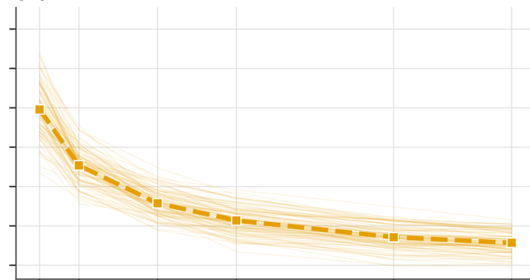
(B) Boosted-Structure
