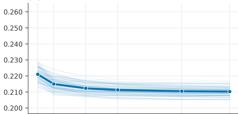
(A) Linear-Structure
