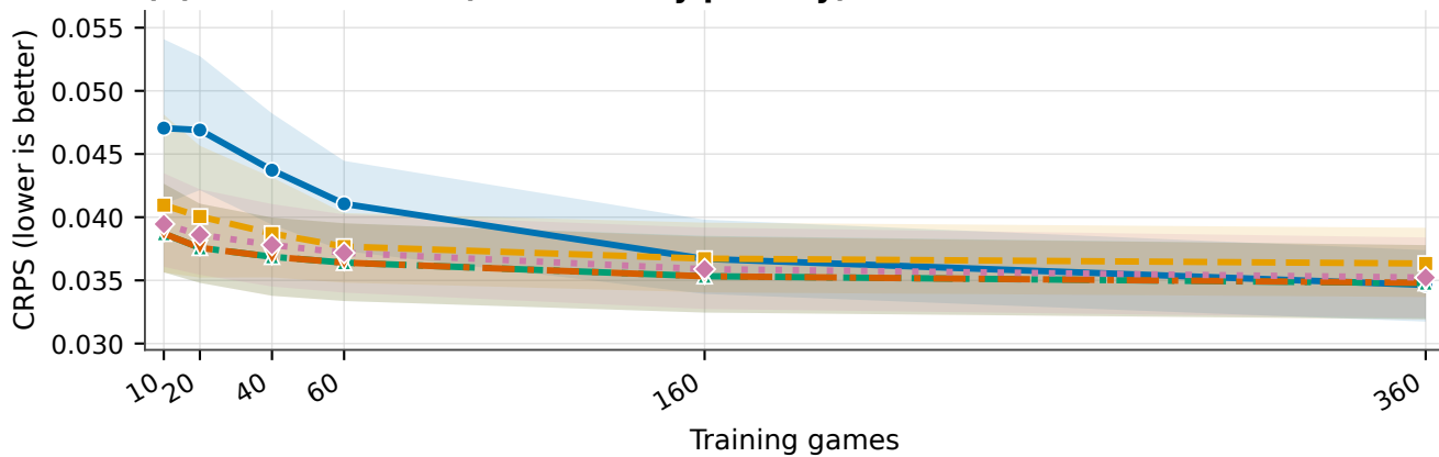
(C) Raw test CRPS (confirmatory primary)
