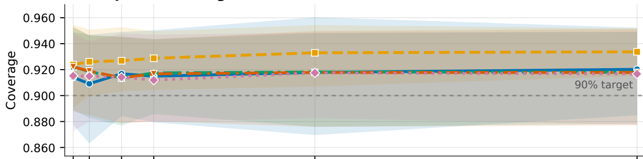
(B) Empirical coverage
