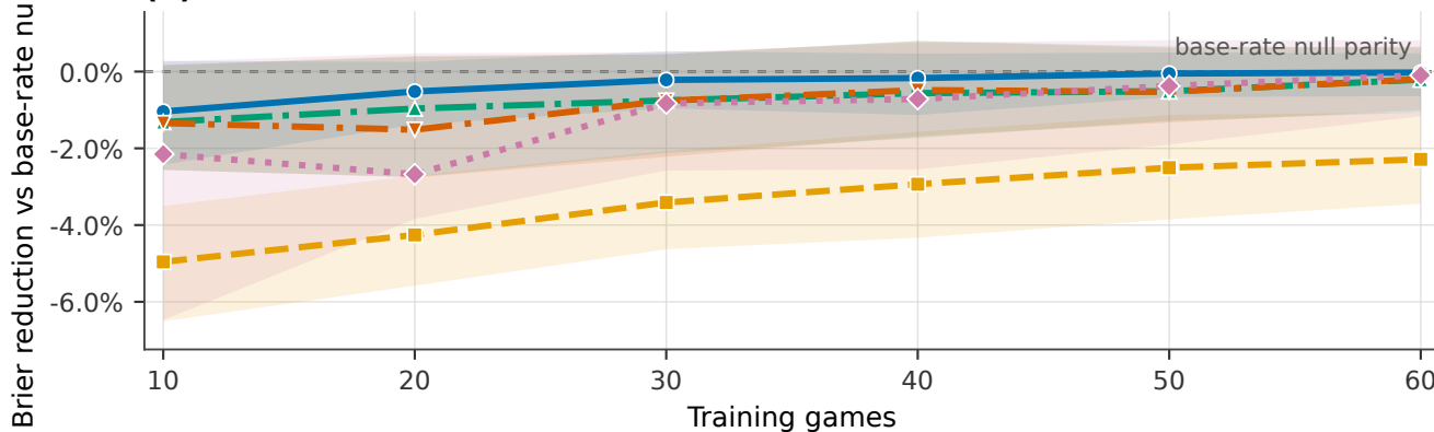
(C) Brier reduction relative to base-rate null
