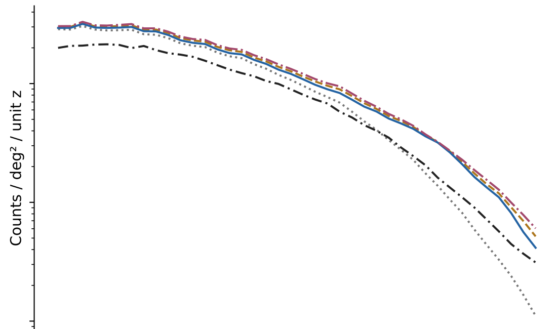
Galactic NGC
