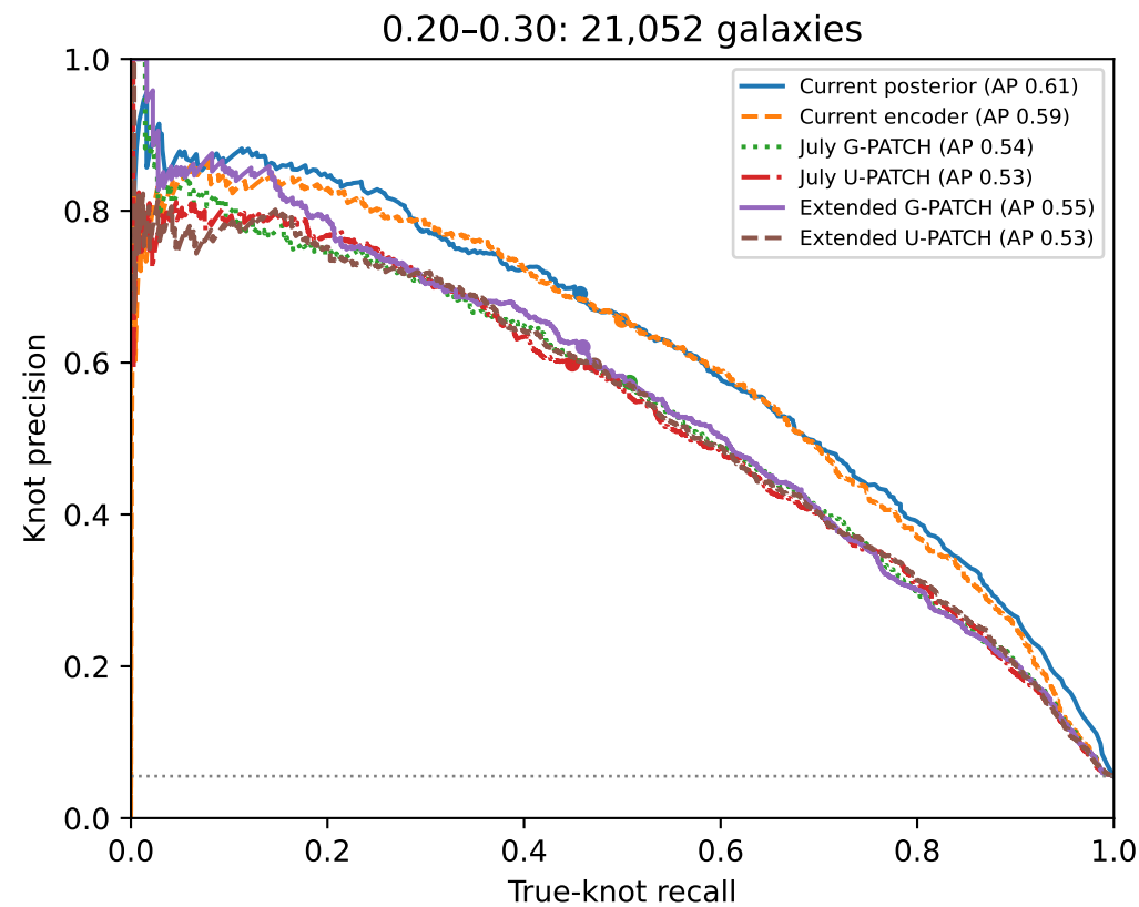
Frozen models on the same exposed ph006 galaxies Dots: original hard decisions; curves: knot probability or smallest-eigenvalue ranking
