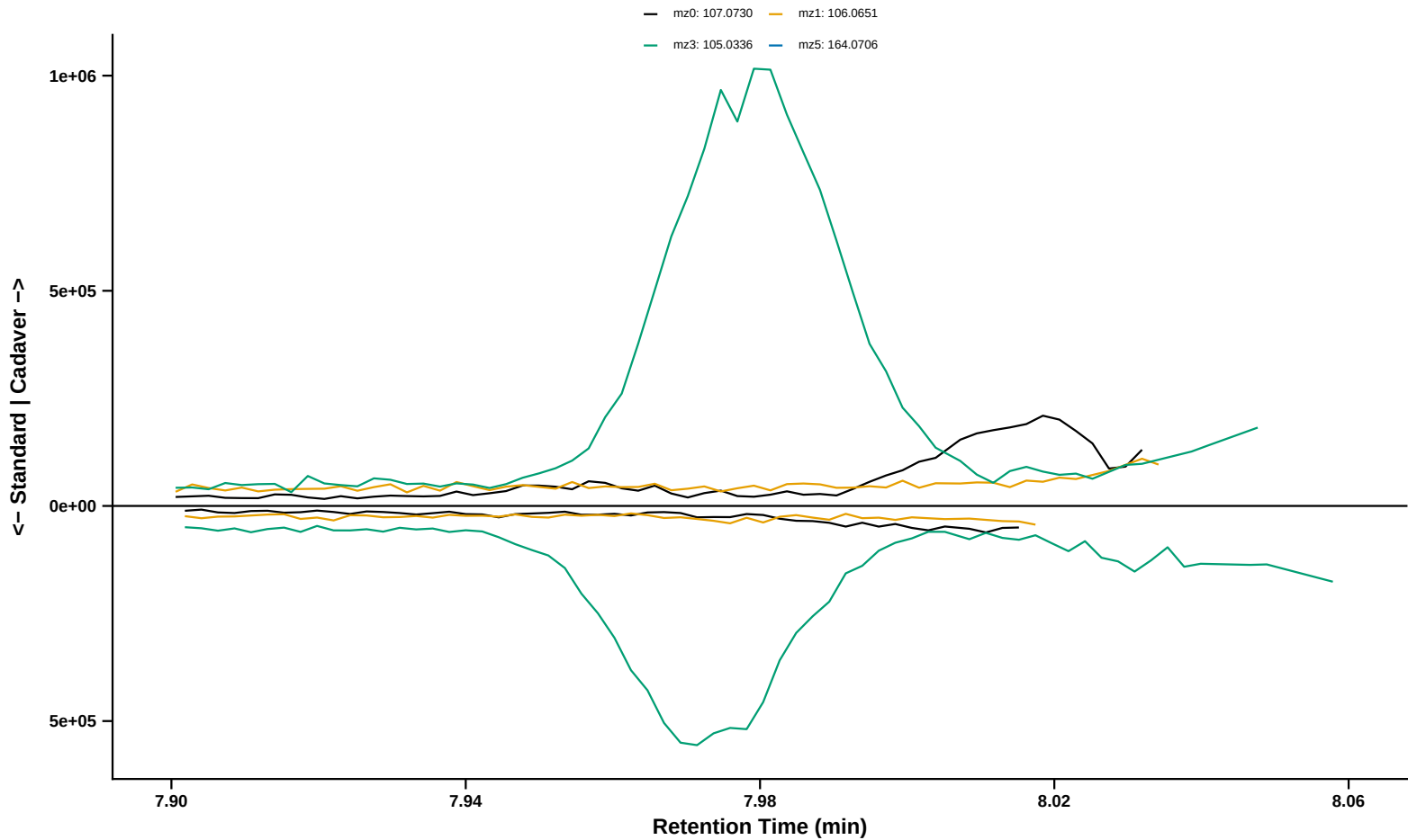
o -Toluidine Sample: BL_08222024_ThyroidTssue_001 | Standard: BP3-1_2 | RT = 8.02 min
