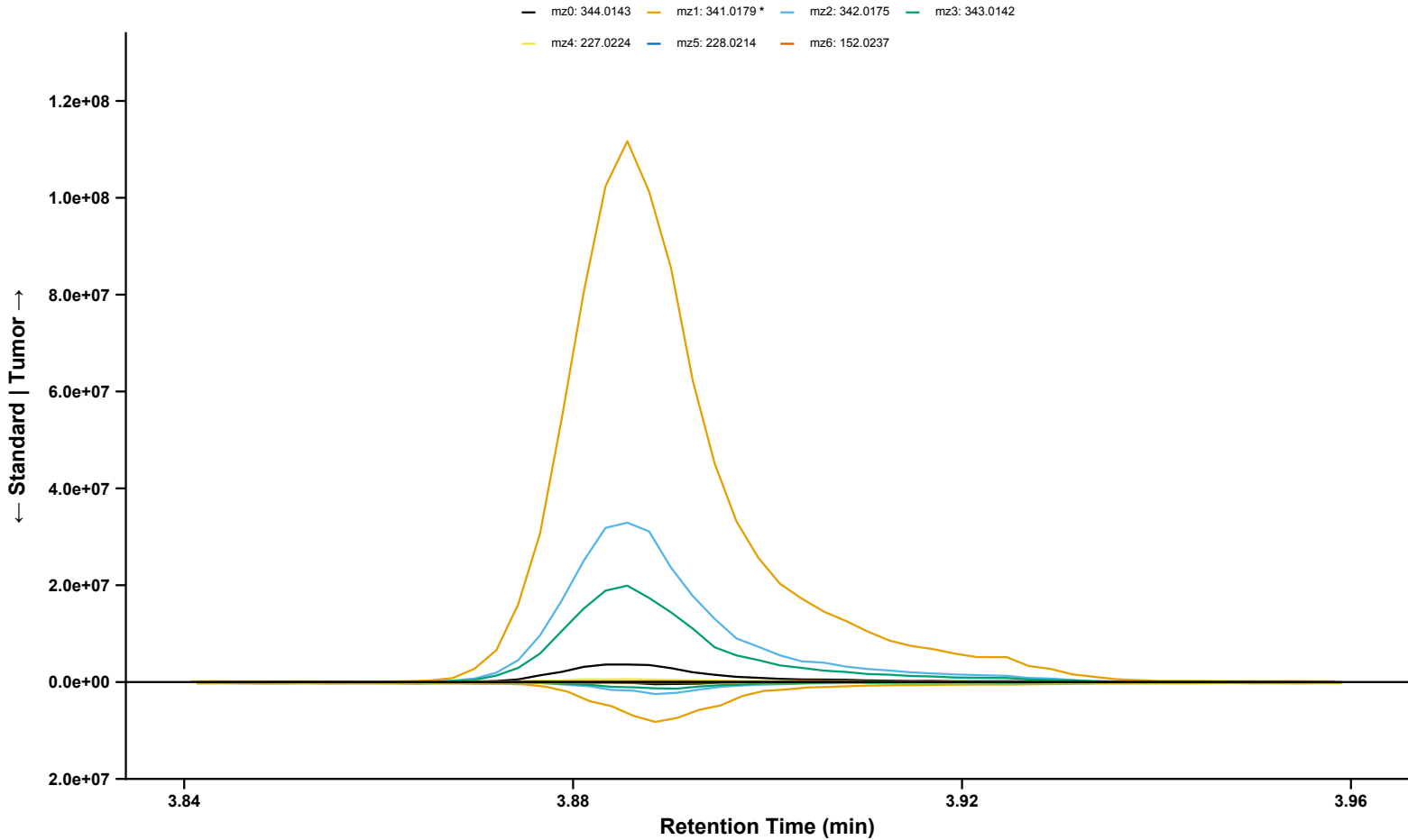
2,4'-Methoxychlor Sample: BL_12082022_003 | Standard: BP2-1_2 | RT = 3.89 min | Analyzed Fragment: mz1
