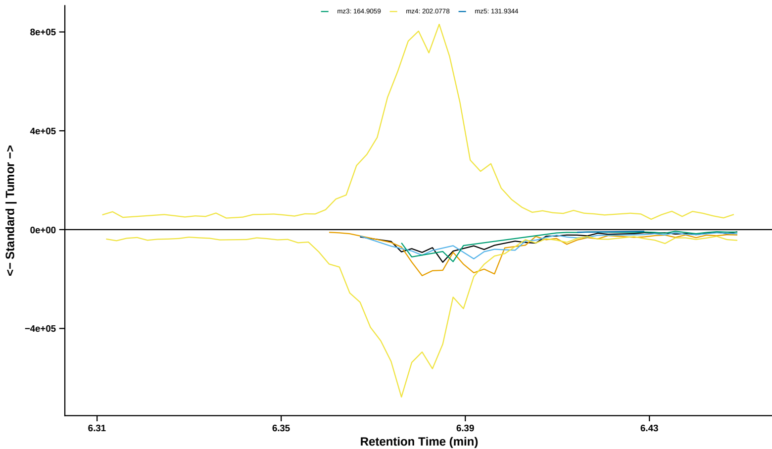
Pentachlorophenol Sample: BL_08222024_ThyroidTssue_005 | Standard: BP1_1 | RT = 6.38 min — mz0: 263.8471 — mz1: 265.8441 — mz2: 267.8412 — mz3: 164.9059 — mz4: 202.0778 — mz5: 131.9344
