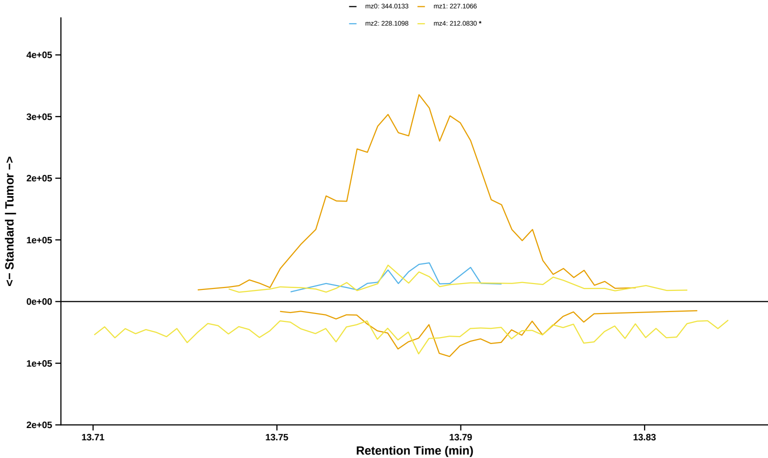
Methoxychlor Sample: BL_12082022_074 | Standard: BP1_1 | RT = 13.78 min | Analyzed Fragment: mz4
