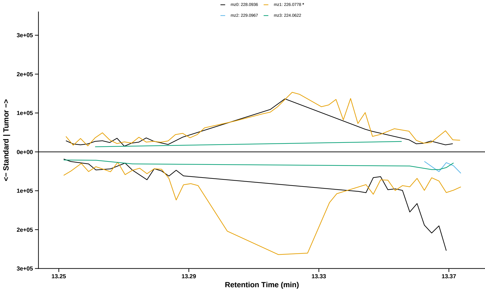
Benz(a)anthracene Sample: BL_12082022_120 | Standard: BP2-1_1 | RT = 13.27 min | Analyzed Fragment: mz1
