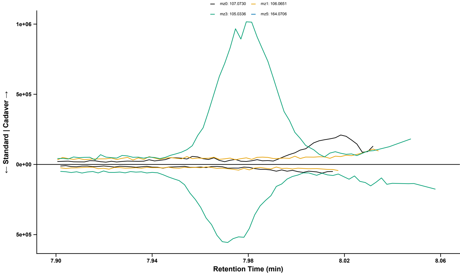
o-Toluidine Sample: BL_08222024_ThyroidTissue_001 | Standard: BP3-1_2 | RT = 8.02 min
