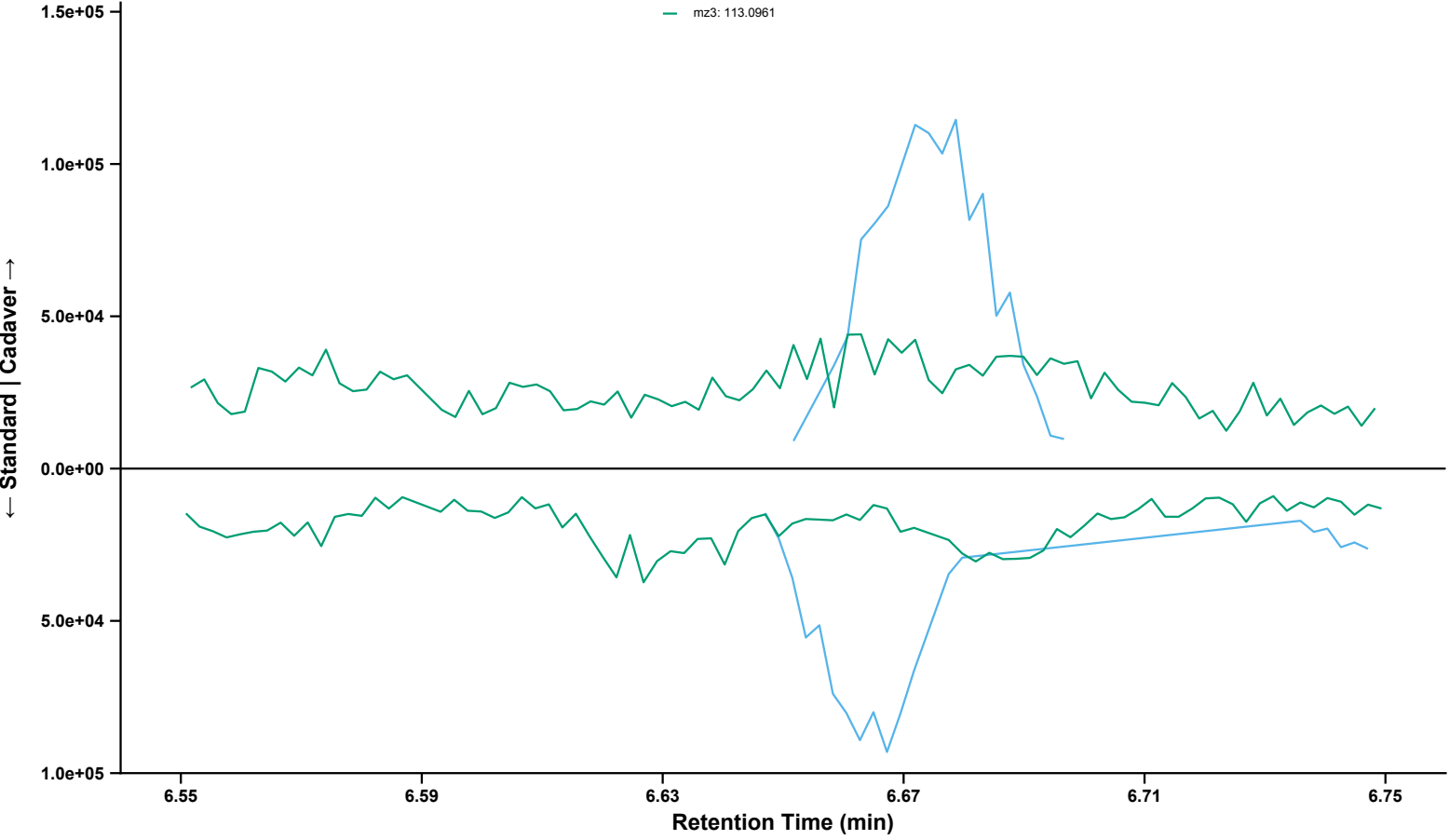
Phenacetin Sample: BL_08222024_ThyroidTssue_005 | Standard: BP2-1_2 | RT = 6.67 min mz0: 179.0941 mz2: 178.0863 mz3: 113.0961
