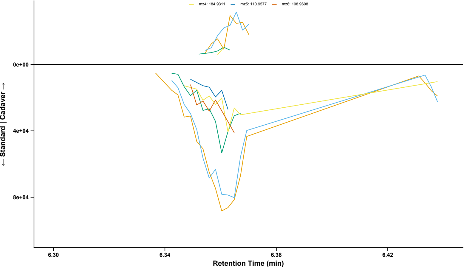
gamma-BHC Sample: BL_08222024_ThyroidTssue_002 | Standard: BP1_1 | RT = 6.37 min mz1: 182.9338 mz2: 180.9370 mz3: 218.9108 mz4: 184.9311 mz5: 110.9577 mz6: 108.9608
