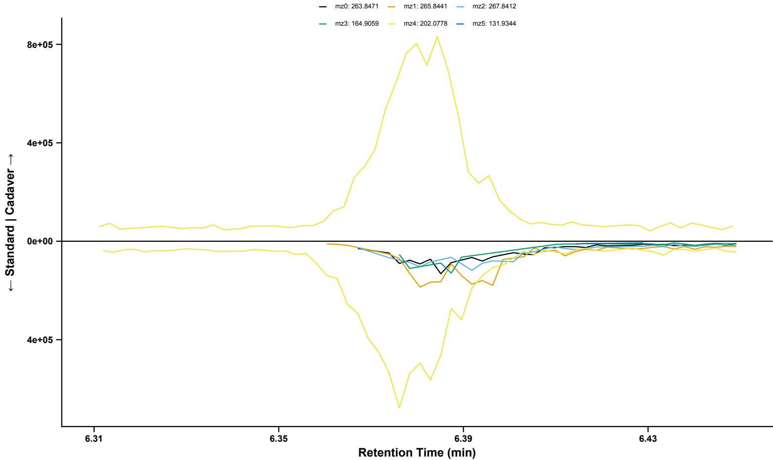
Pentachlorophenol Sample: BL_08222024_ThyroidTissue_005 | Standard: BP1_1 | RT = 6.38 min
