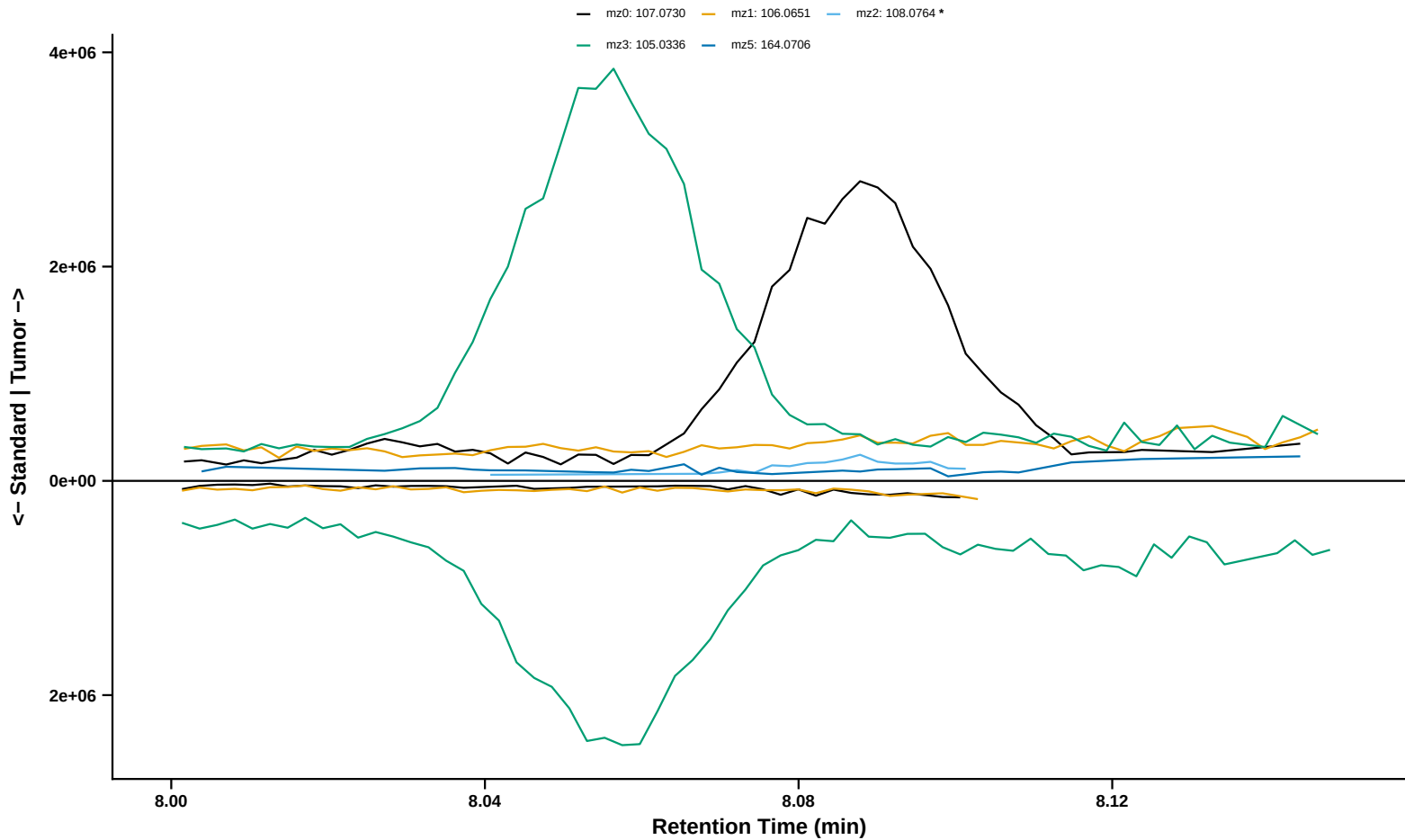
o-Toluidine Sample: BL_12082022_034 | Standard: BP3-1_2 | RT = 8.08 min | Analyzed Fragment: mz2
