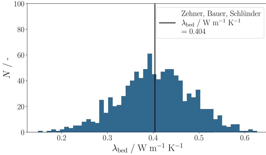
Figure 4.2: The radial heat conductivity of the packed bed follows a normal distribution with its mean calculated by the correlation of Zehner et al. [31] and a standard deviation of \sigma = 0.08 \text{ W m}^{-1} \text{ K}^{-1} , shown for 1000 sampling points.
