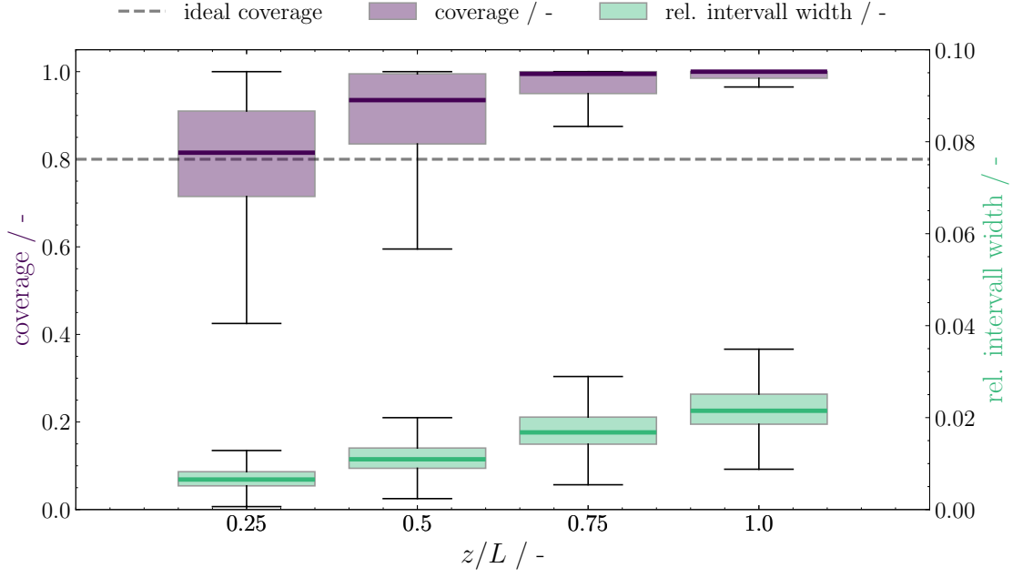
Figure 5.10: Coverage (purple) and relative interval width (green) for the temperature quantiles of the NARX models in the naive physics-consistent framework. The ideal intended coverage (dashed line) lies at 0.8.
