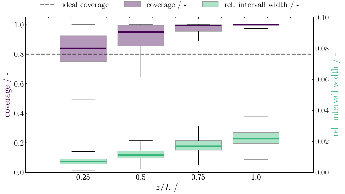
Figure 5.11: Coverage (purple) and relative interval width (green) for the temperature quantiles of the NARX models in the fully physics-consistent framework. The ideal intended coverage (dashed line) lies at 0.8.
