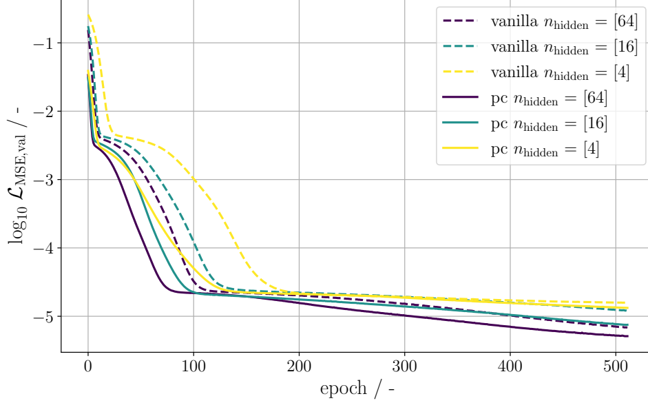
Figure 5.1: The validation loss calculated as MSE \mathcal{L}_{\text{MSE, val}} during the training of the vanilla NARX (dashed line) and the physics-constrained NARX (solid line). The three data rows indicate one hidden layer with 64, 16 and 4 hidden neurons each. The physics-constrained NARX converges visibly faster than the vanilla NARX.
