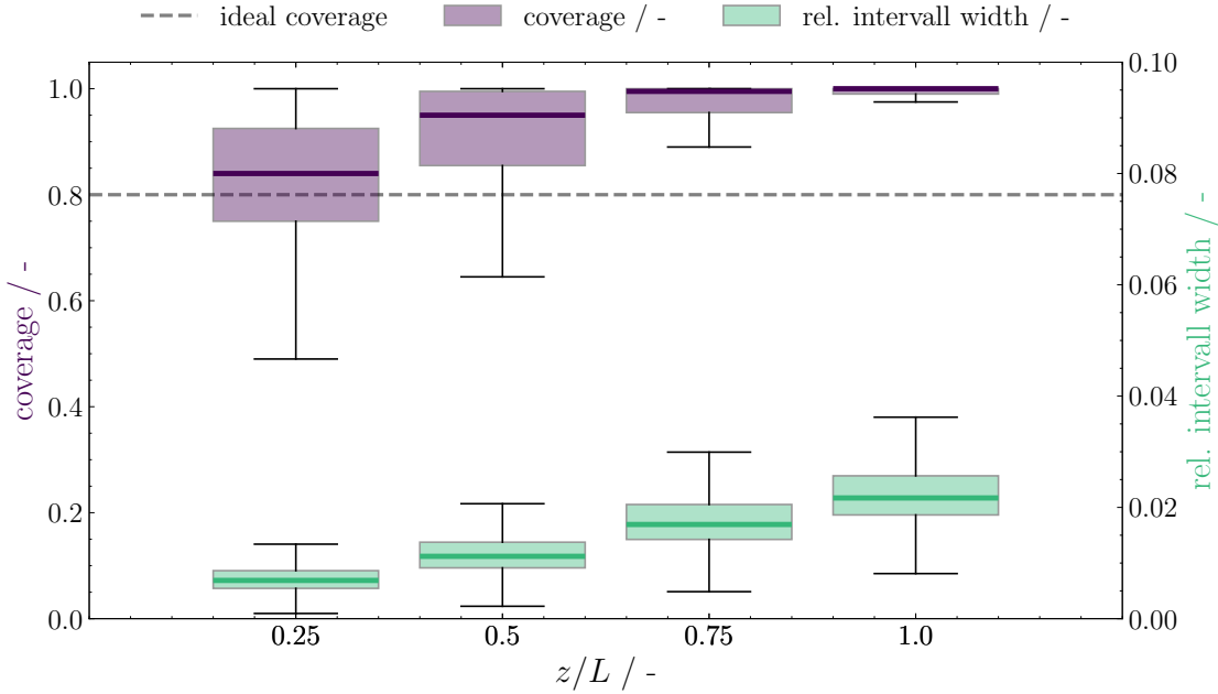
Figure 5.11: Coverage (purple) and relative interval width (green) for the temperature quantiles of the NARX models in the fully physics-consistent framework. The ideal intended coverage (dashed line) lies at 0.8.
