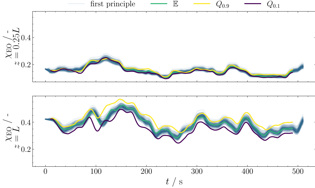
Figure 5.8: Forward simulation of the pc NARX framework with physics-constrained activation for 480 s. The fully physics-constrained framework exhibits a minor improvement to the vanilla NARX framework.
