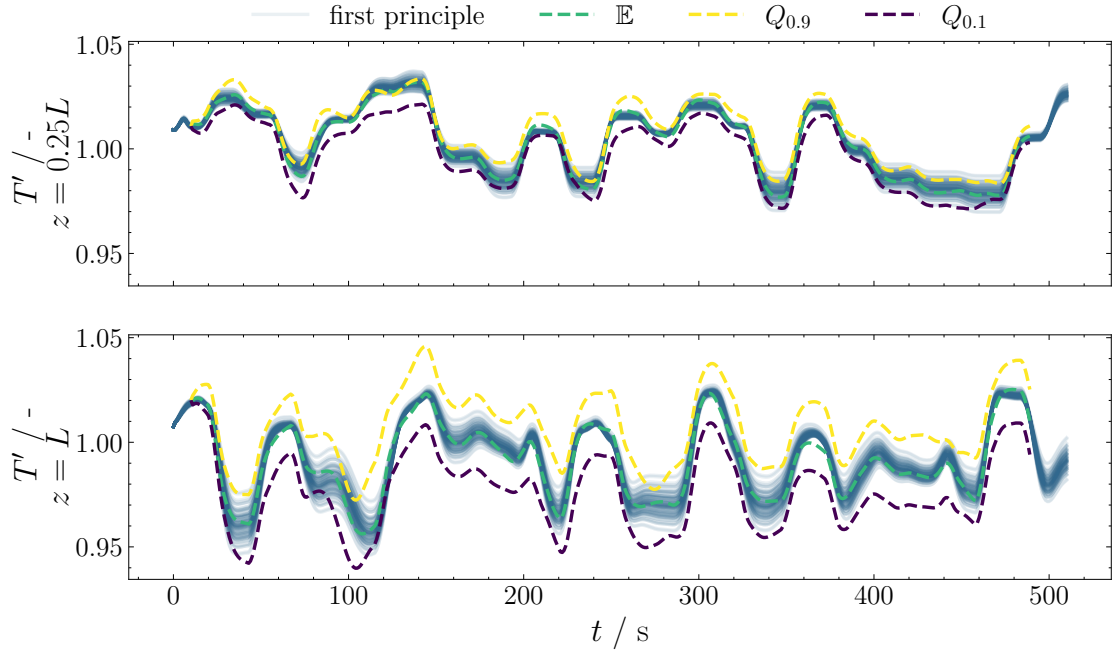
Figure 5.5: Forward simulation of the vanilla-NARX framework without physics-constrained activation for 480 s. The scaled temperature T' is shown for two measurement positions z = 0.25L and z = L . 100 first principle system trajectories are displayed as test data (light blue) for MC sampled parameters.
