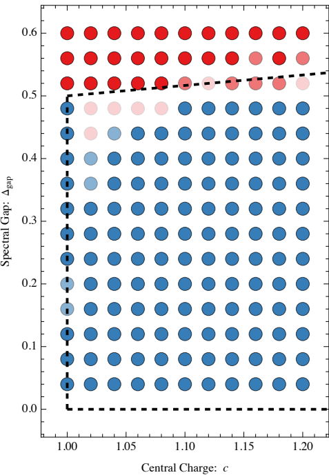
\Delta_{\max}=4 Spectra Truncated to \Delta_{\max}=3
