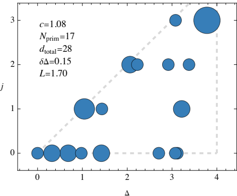
Spectrum After Optimization: c=1.08 , \Delta_{\text{gap}}=0.32
