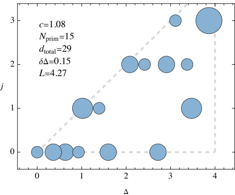
Spectrum After Optimization: c=1.08 , \Delta_{\text{gap}}=0.36
