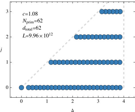
Spectrum Prior to Optimization: c=1.08 , \Delta_{\text{gap}}=0.28
