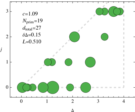
Spectrum After Optimization: c=1.09 Candidate
